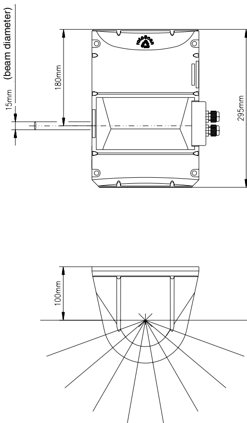
Figure 5.1: Scanning plane
