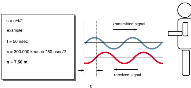
Figure 1.3: Phase measurement
